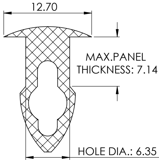
SECTION Y-Y
